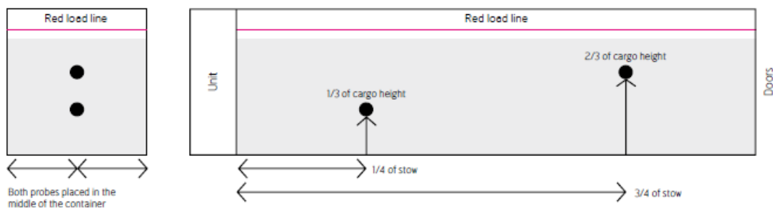
Correct positioning of temperature recorders:
